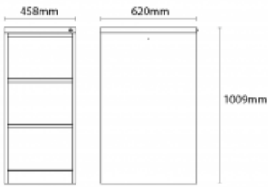
3 DRAWER FOOLSCAPE CABINET (FCLM3F)
