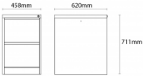
2 DRAWER FOOLSCAPE CABINET (FCLM2F)
